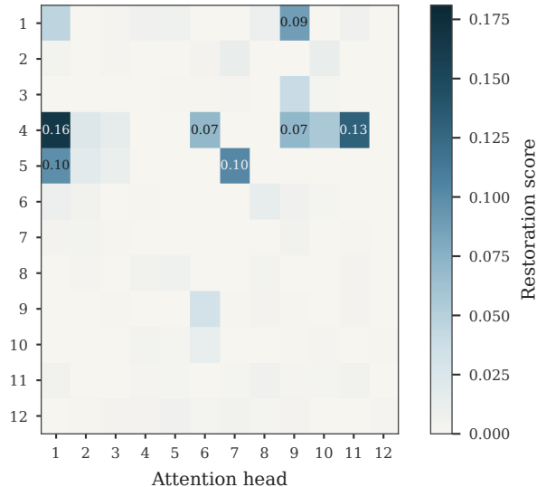
Recovery (Gutenberg)
